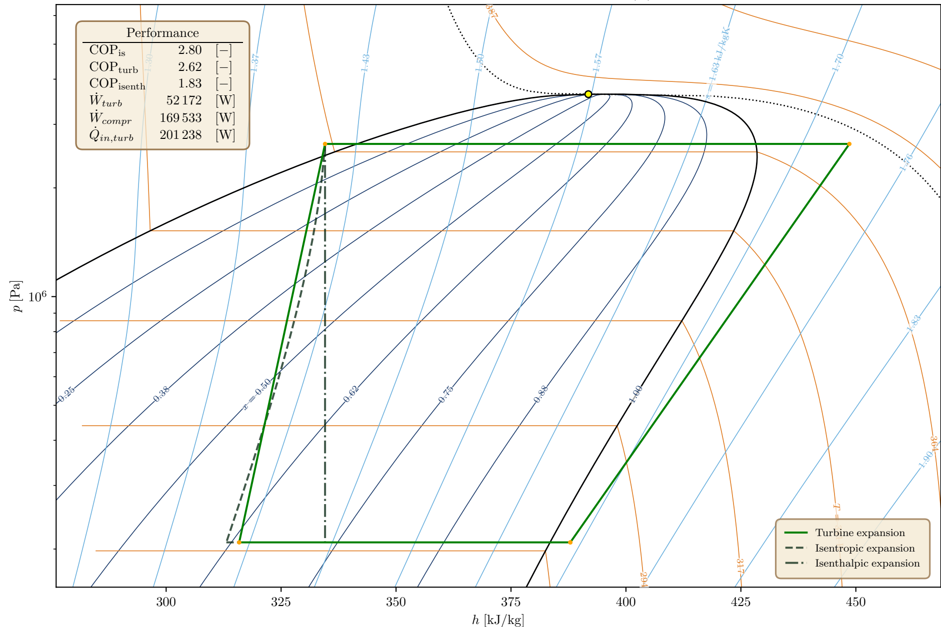
Conceptual Heat Pump Cycle – R1234ze(E)
